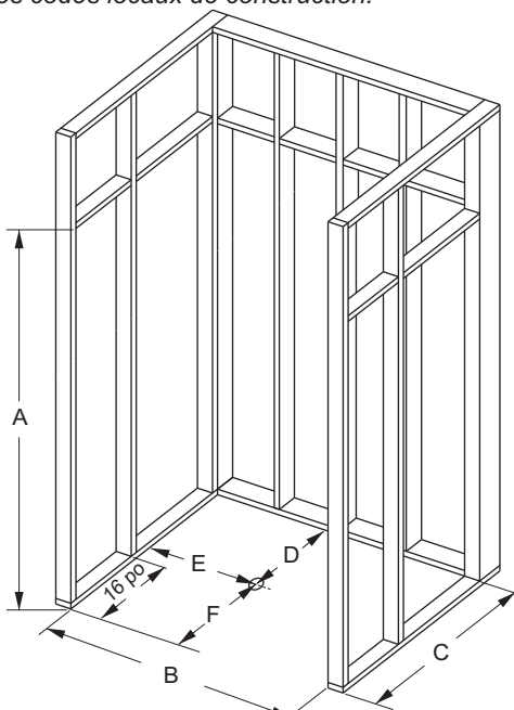
ILLUSTRATION 1 - LAYOUT DIMENSIONS
