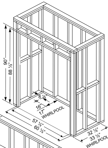
FIGURE 1 - LAYOUT DIMENSIONS
