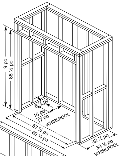
ILLUSTRATION 1 - DIMENSIONS
