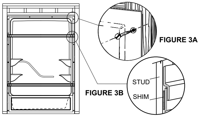
FIGURE 3 - FASTENING WITH DRYWALL SCREWS
